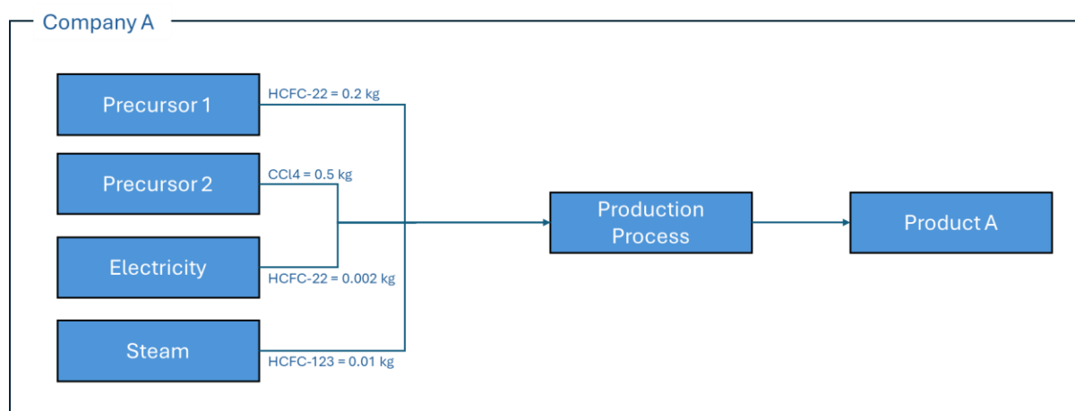
Figure 11: Simplified example of an ODP calculation for a chemical process with ODP mass emission flows.
