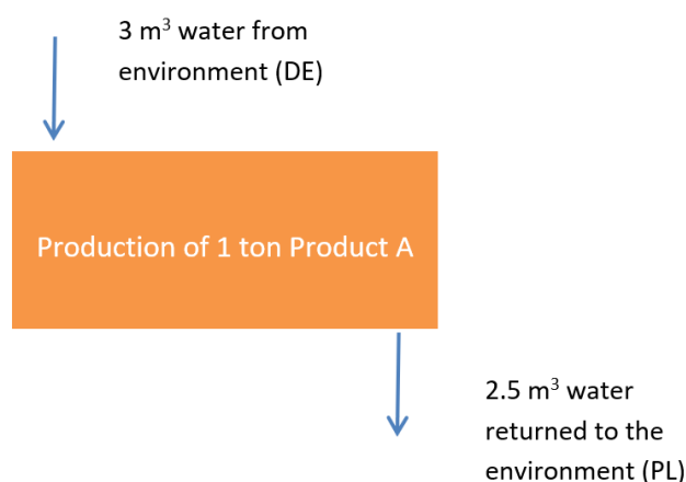
Figure 15: Example 2: Water scarcity impact when input water country of origin is different from output water.
