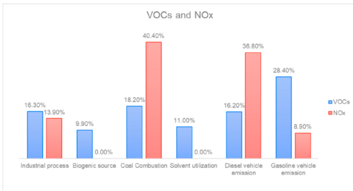
Figure 12: Representation of the six main sources of VOCs and \text{NO}_x in a typical industrial city in China.
