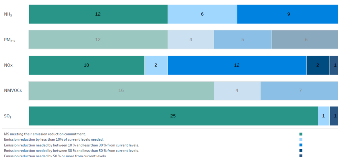
Figure 7: Number of Member States that had met their national emission reduction commitments for the five main pollutants for 2030.
