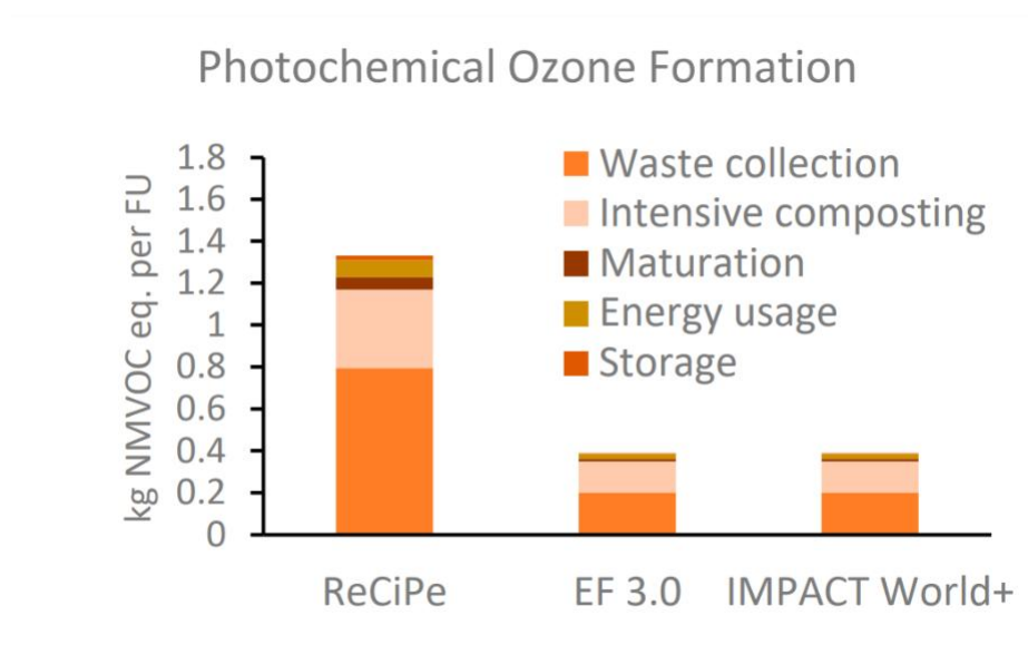
Figure 17: Comparison of photochemical ozone formation values (in kg NMVOC eq.) between the three methods: ReCiPe, EF 3.0 and IMPACT World+.
