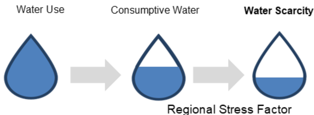
Figure 6: Definition of water scarcity footprint
