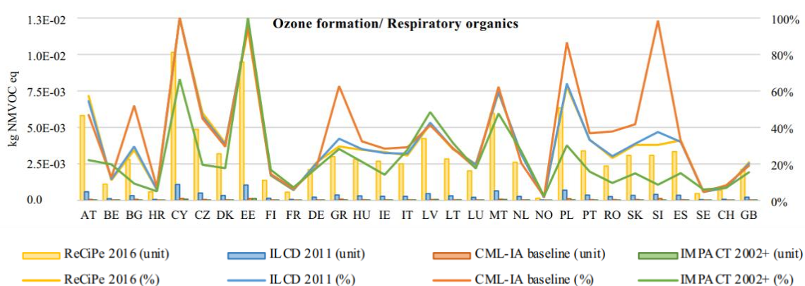
Figure 18: Comparison of photochemical ozone formation values (in kg NMVOC eq.) between the four methods: ReCiPe 2016, ILCD 2011, CML-IA baseline and IMPACT 2002+
