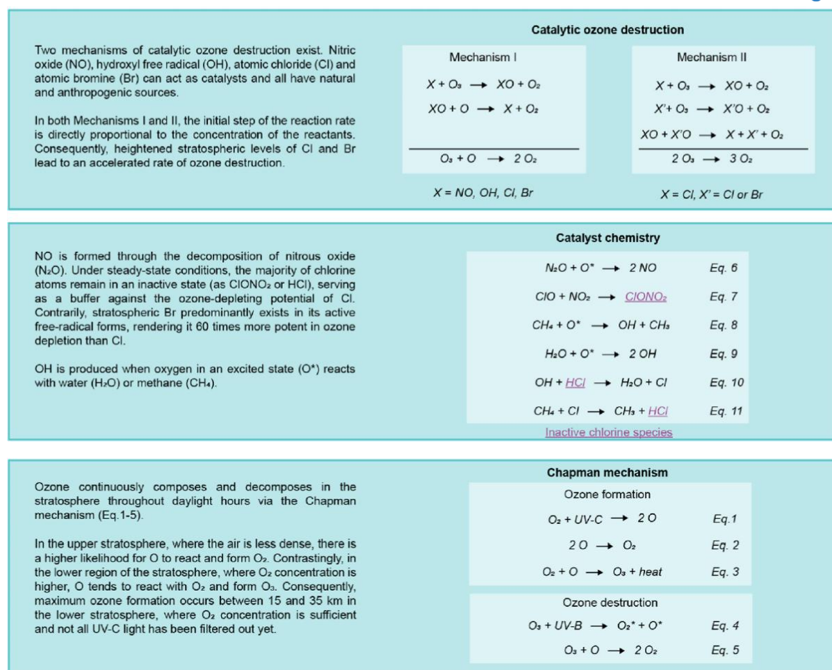
Figure 9: Summary of stratospheric ozone chemistry.
