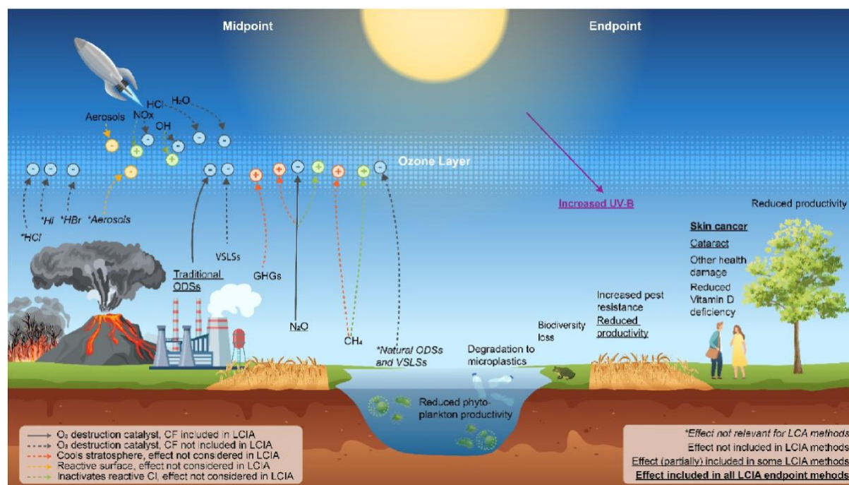
Figure 10: Summary of limitations and challenges related to midpoint and endpoint characterization.
