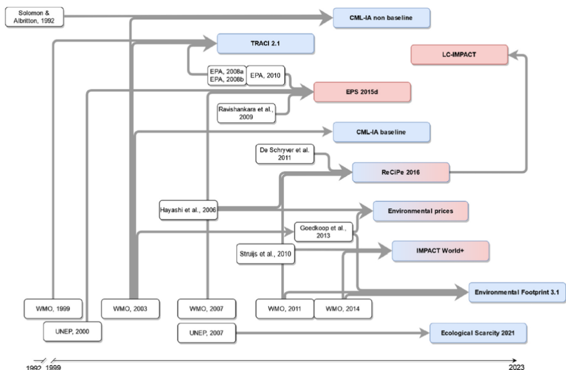
Figure 16: Overview of existing LCIA methods considering ODP in midpoint (blue ovals) and endpoint (red ovals) methods. White ovals represent data sources for ODP and model assumptions.
